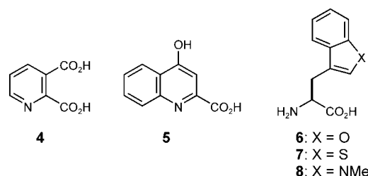
Scheme 2. Kynurenine pathway metabolites ( 4 and 5 ) and tryptophan analogues ( 6–8 ).
