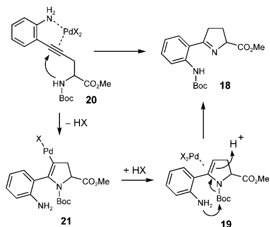
Scheme 6. Mechanism of pyrroline formation.
