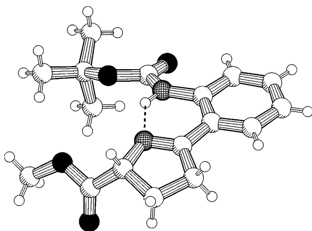
Figure 1. PLATON drawing of the X-ray crystal structure of imine 18 .
