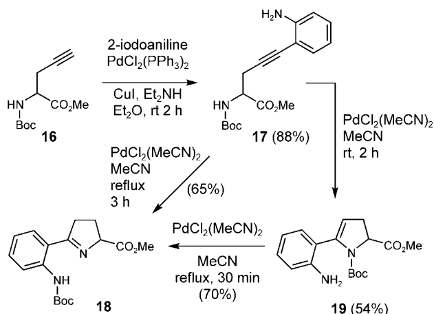
Scheme 5. Unexpected pyrroline formation.
