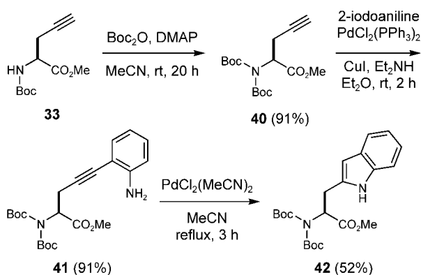
Scheme 10. Pd-catalyzed cyclization to isotryptophan.
