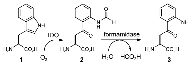
Scheme 1. The first steps in the kynurenine pathway.
