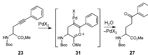
Scheme 7. Mechanism of alkyne hydration.
