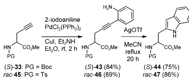
Scheme 11. Ag-catalyzed cyclization to isotryptophan.
