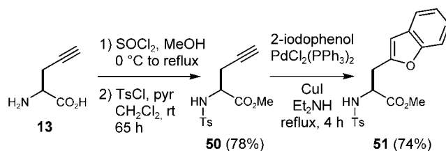
Scheme 13. One-pot coupling/cyclization to benzofuran derivative 51 .
