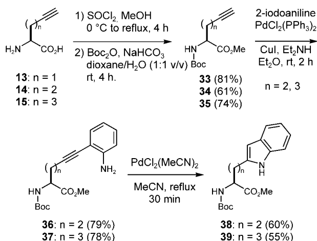
Scheme 9. Synthesis of isotryptophan derivatives.
