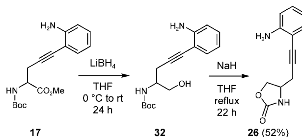
Scheme 8. Formation of oxazolidinone 26 .
