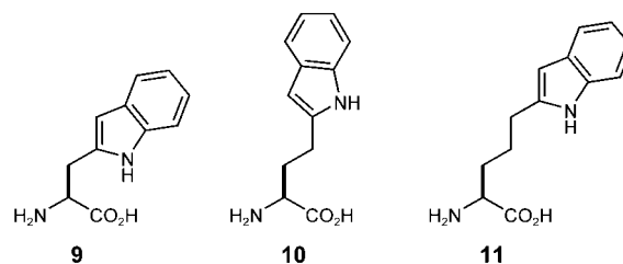
Scheme 3. Targeted tryptophan derivatives.
