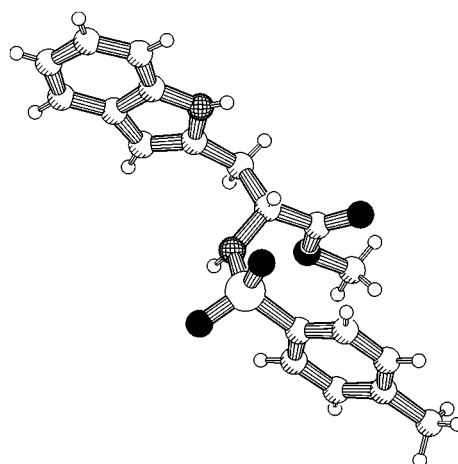
Figure 2. PLATON drawing of the X-ray crystal structure of 47 .
