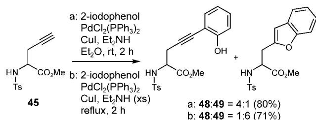
Scheme 12. Synthesis of benzofuran analogue 49 .
