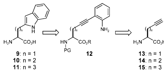
Scheme 4. Retrosynthesis of isotryptophans.
